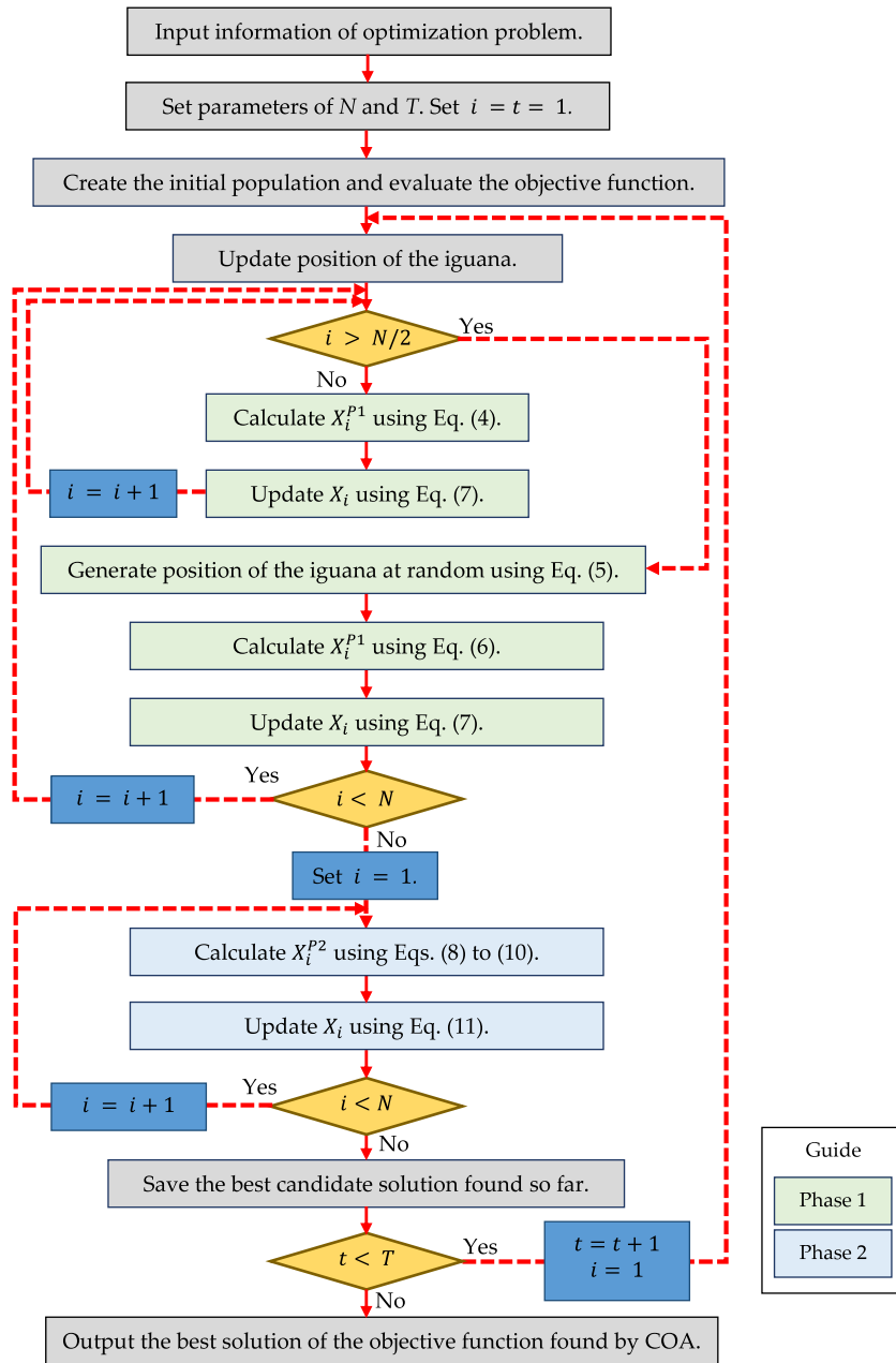
Fig. 4. The flowchart of the COA.
